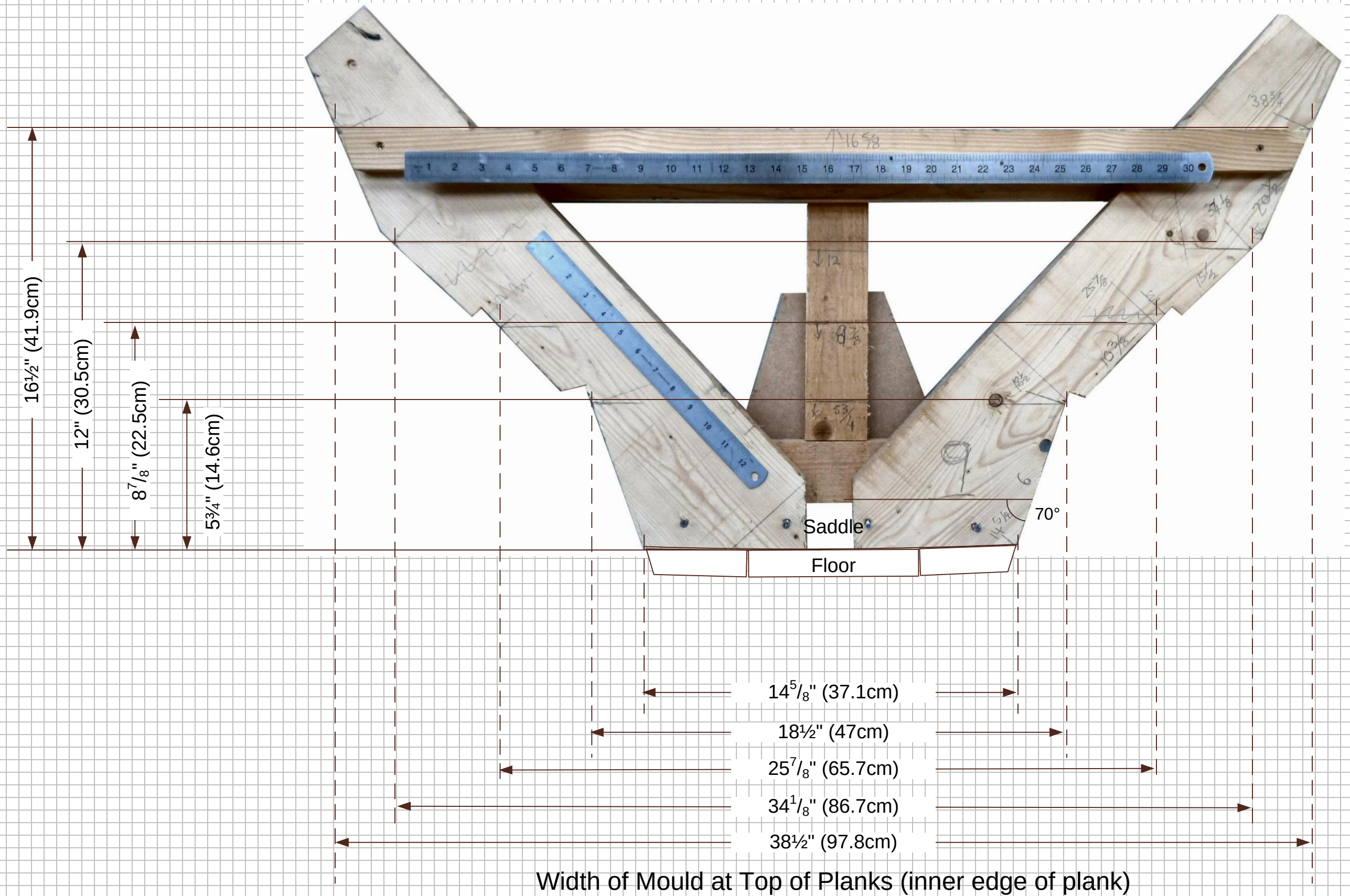
Figure 77 - Mould Dimensions at Station 9.
