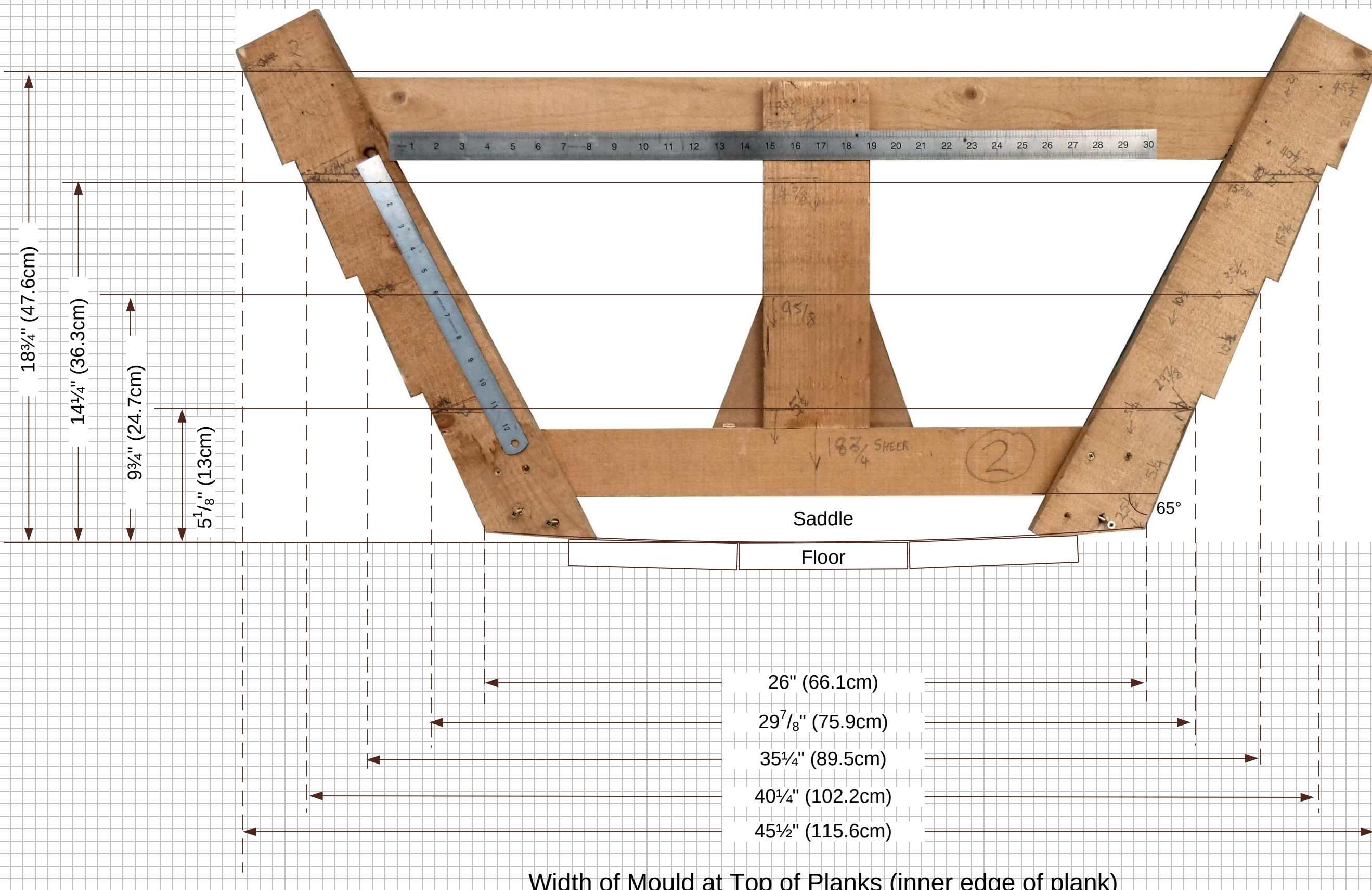
Figure 72 - Mould Dimensions at Station 2.
