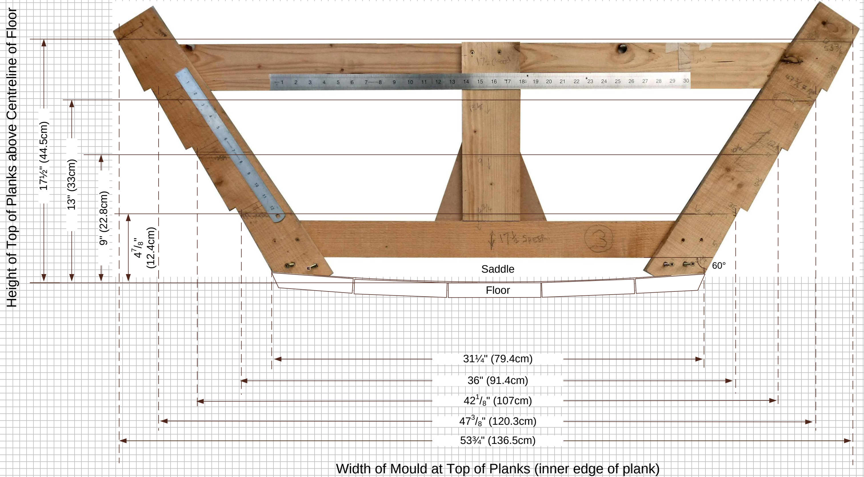
Figure 73 - Mould Dimensions at Station 3.
