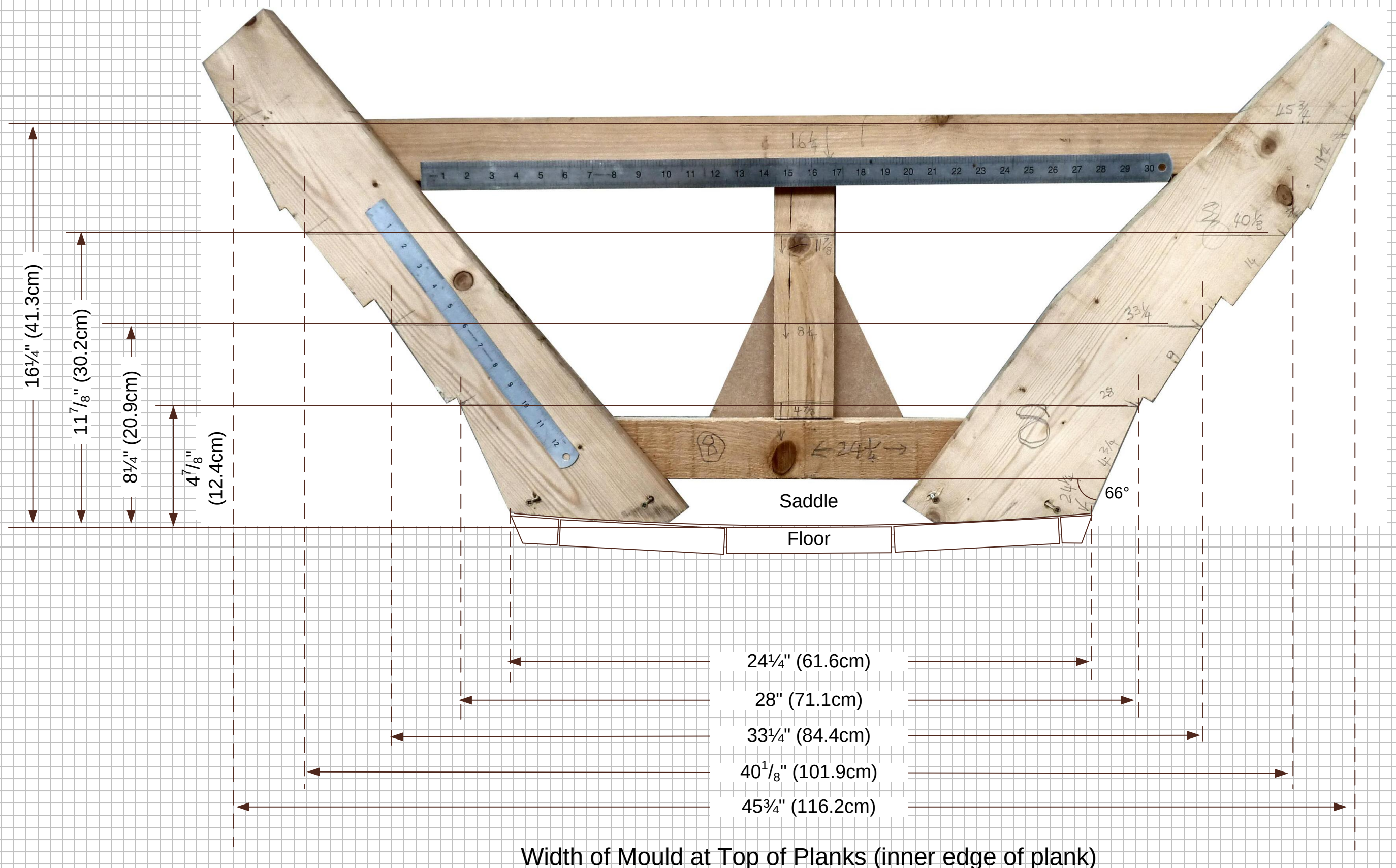
Figure 76 - Mould Dimensions at Station 8.
